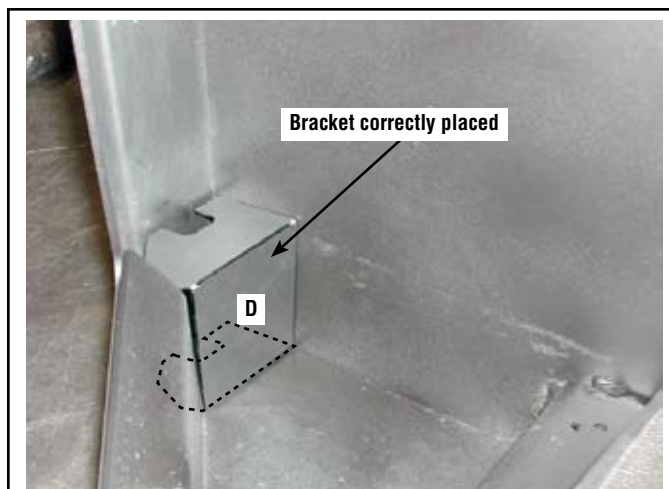
Figure 3 - Log Support Bracket
