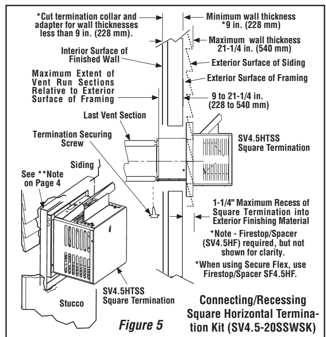
Installing Square Horizontal Termination (SV4.5HTS) or Short Square Horizontal Termination (SV4.5HTSS)
