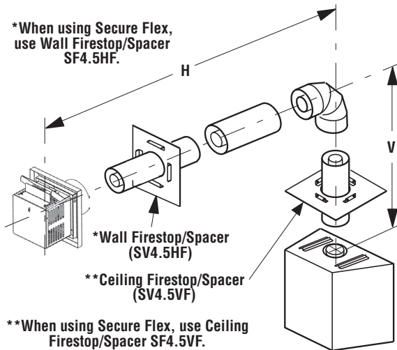
Figure 9 - Top Vent - ONE 90 DEGREE ELBOW - ELBOW CONNECTION NOT DIRECTLY AT APPLIANCE
